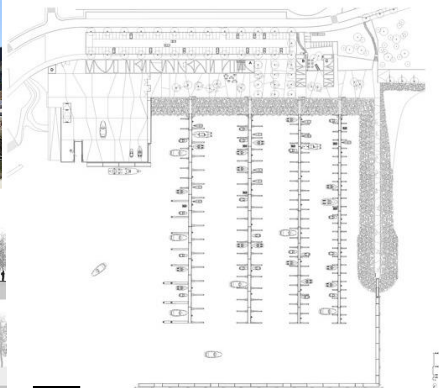
SITE PLAN
